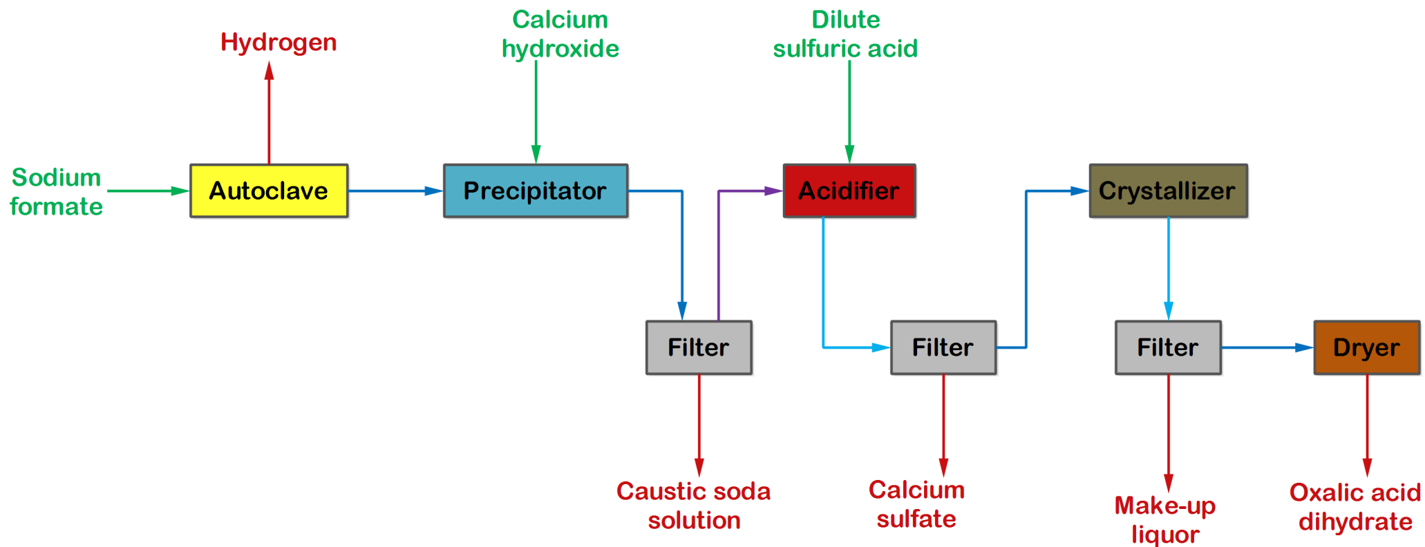
Figure: Manufacture of Oxalic acid from Sodium formate
